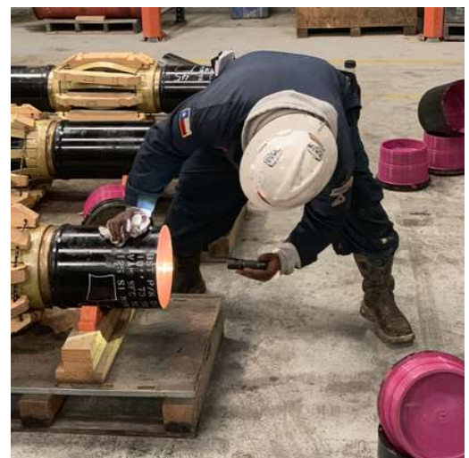
Visual inspection of a premium connection, box end.
